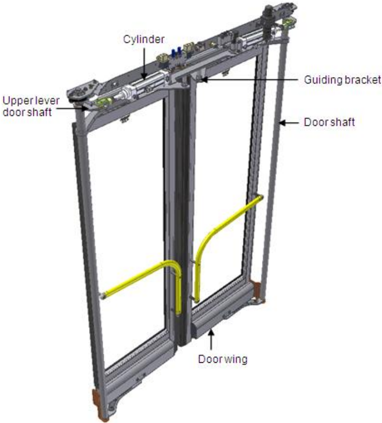
Figure: Door system description
